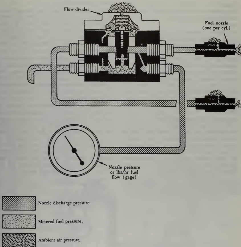
FIGURE 3-34. Flow divider.
